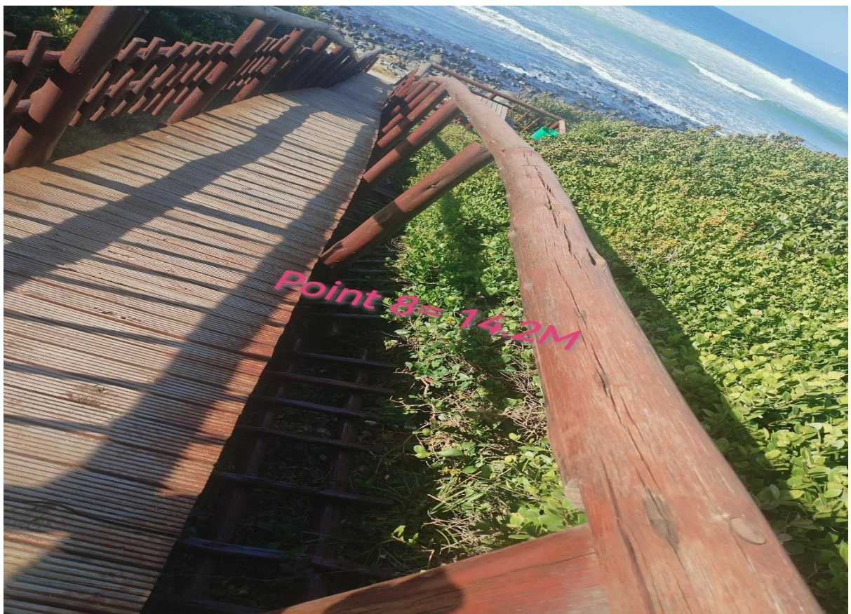
Point 8: Replacement of slats and stabilise the wobbly decking Dimensions for slats - (H x 120cm) (L x 14.2m) Dimensions for the decking- (W x 123cm) (L x 14.2m)
