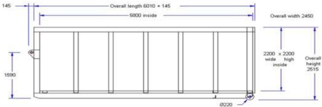
28m 2 Roll-on Bin Dimensions
