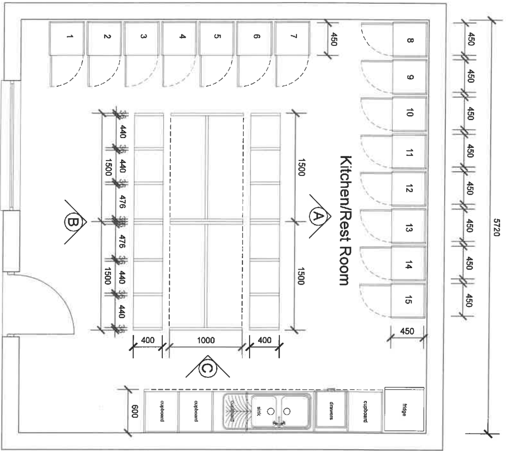
Floor Plan Scale - 1:50
